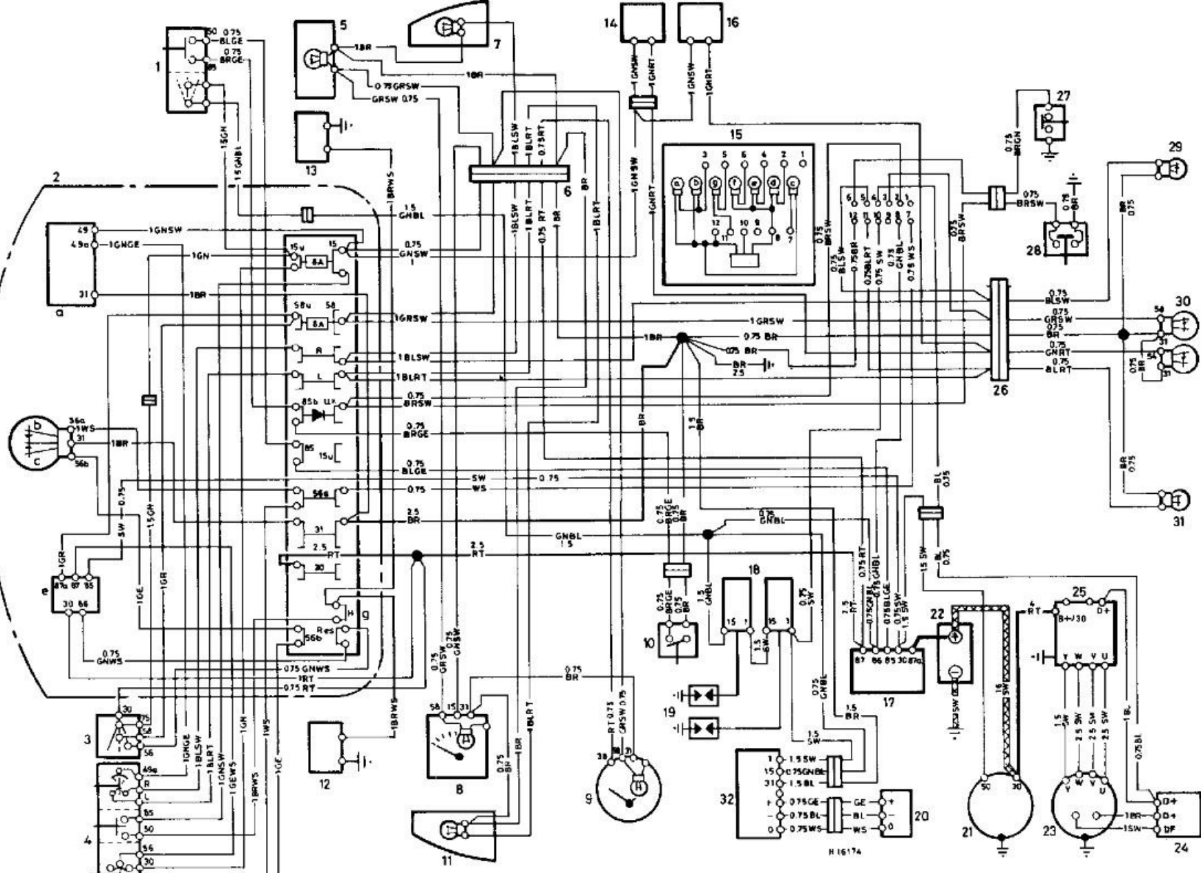
Wiring diagram - 1983 to 1984 R80RT and 1981 on R100RT, R100RS models
